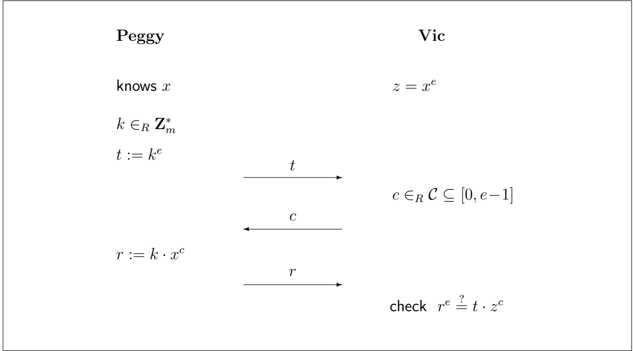
Fig. 2. The Guillou-Quisquater (GQ) protocol for proving knowledge of an e -th root x modulo m of a given element z \in \mathbf{Z}_m^* .
