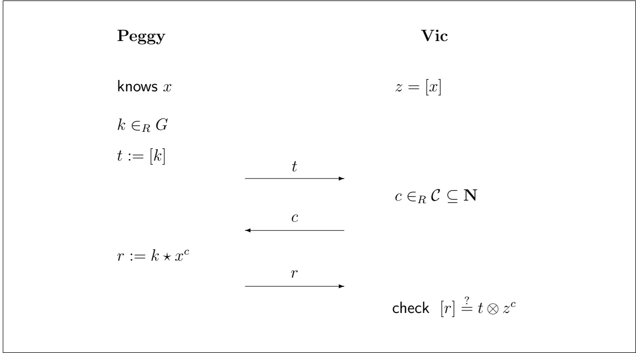
Fig. 3. Main protocol: Proof of knowledge, for a given value z , of a value x such that z = [x] , where x \mapsto [x] is a (one-way) group homomorphism.
