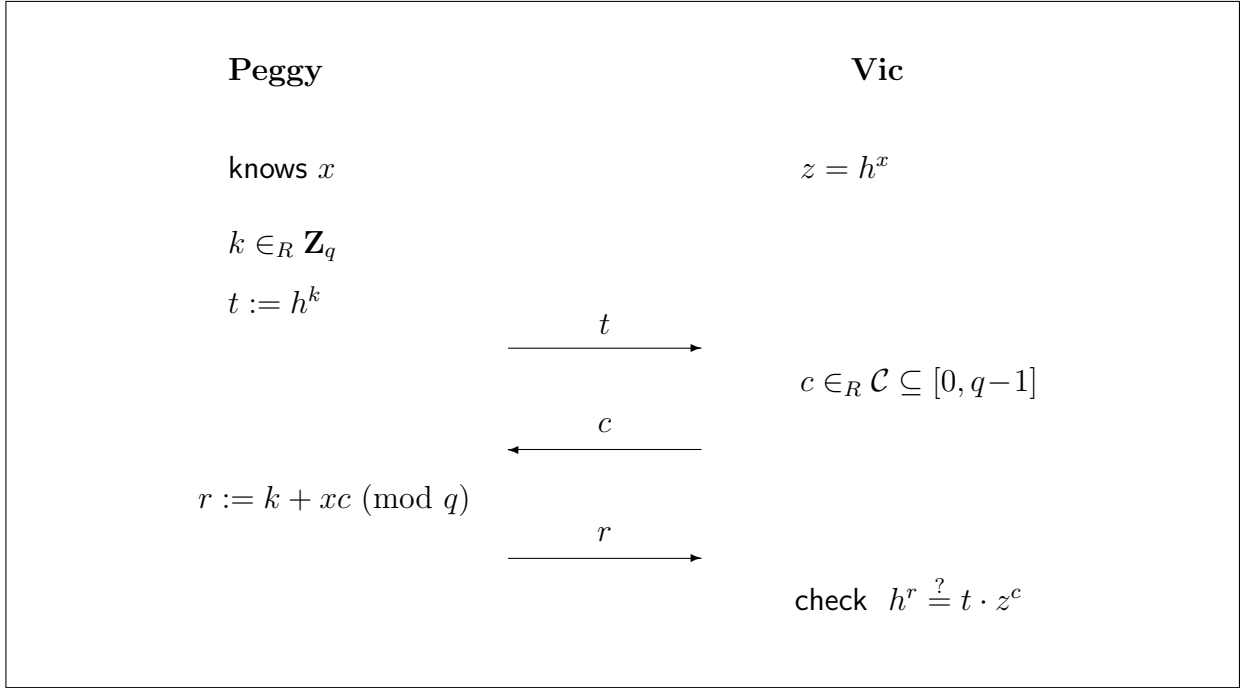
Fig. 1. The Schnorr protocol for proving knowledge of a discrete logarithm x of an element z = h^x in the group H .
