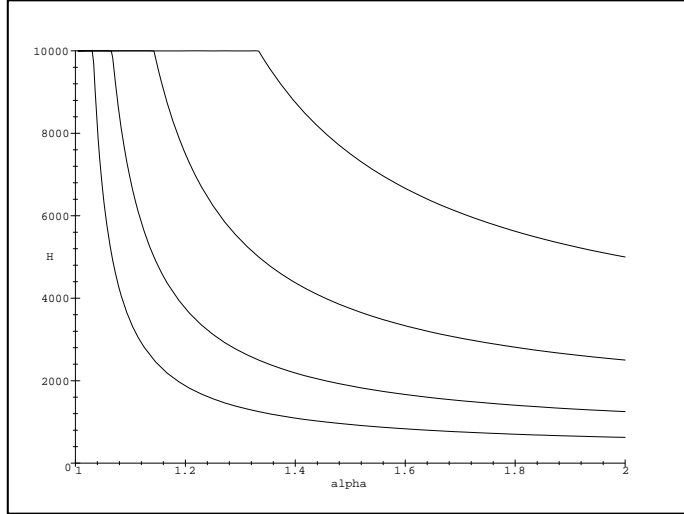
Figure 1: Rényi entropy H_\alpha(X_\beta) as function of \alpha between 1 and 2. The random variables X_\beta for \beta = 16, 8, 4, 2 (from below) are defined as in Example 2 with n = 10000 . The graph shows that, together with Theorem 8, Rényi entropy of order \alpha close to 1 can yield much better bounds on smooth entropy than Rényi entropy of order 2.
