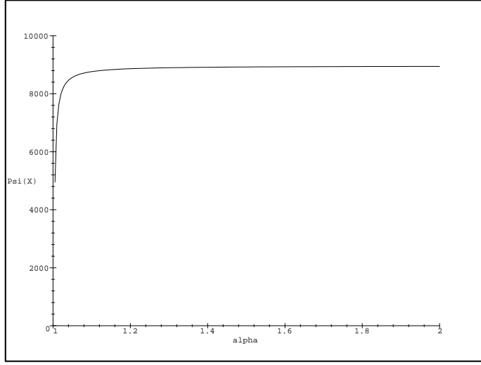
Figure 2: The dependence of the lower bound for \Psi(X) on the order \alpha of Rényi entropy. The graph shows the lower bound of Theorem 8 on the smooth entropy \Psi(X) within 2^{-s}/\ln 2 with probability 1 - 2^{19} that can be deduced from H_\alpha(X) \geq 9000 as a function of \alpha . Note the sharp decrease with \alpha \rightarrow 1 . (See also Example 3.)
